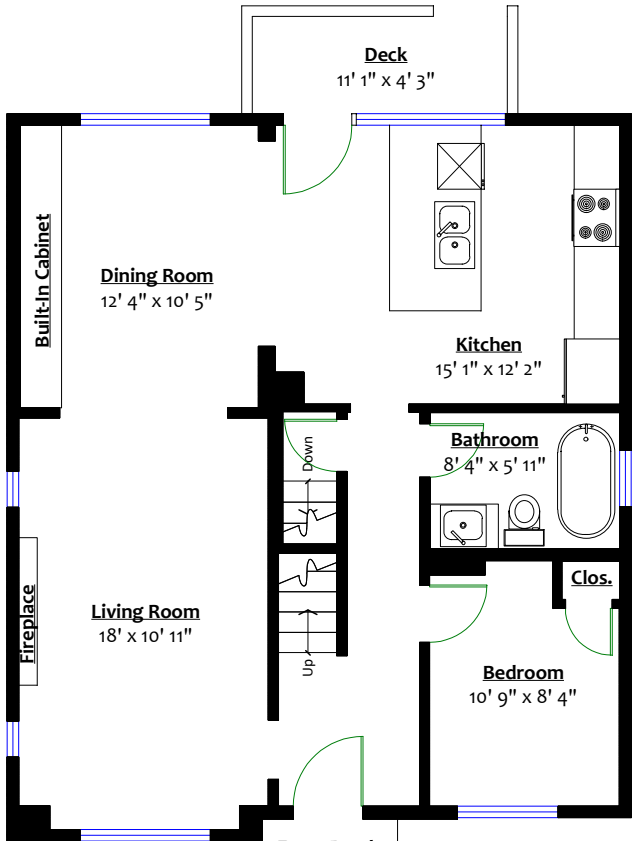
MAIN LEVEL Floor Area: 850 Sq. Ft. Ceiling Height: 8' 3"
