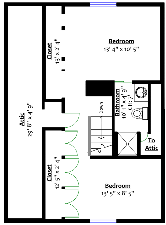
UPPER LEVEL Floor Area: 685 Sq. Ft. Ceiling Height: ' 6"
